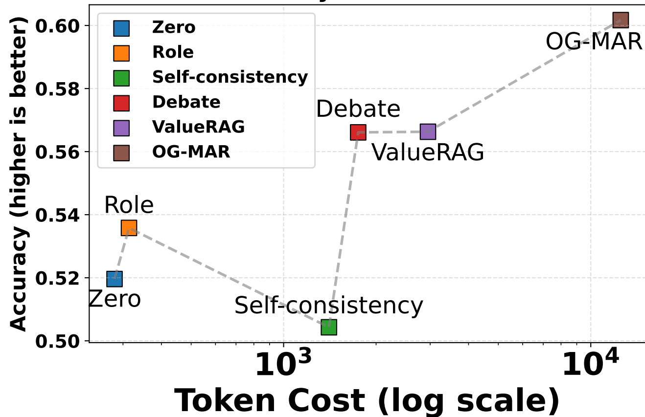
Accuracy vs Token Cost
